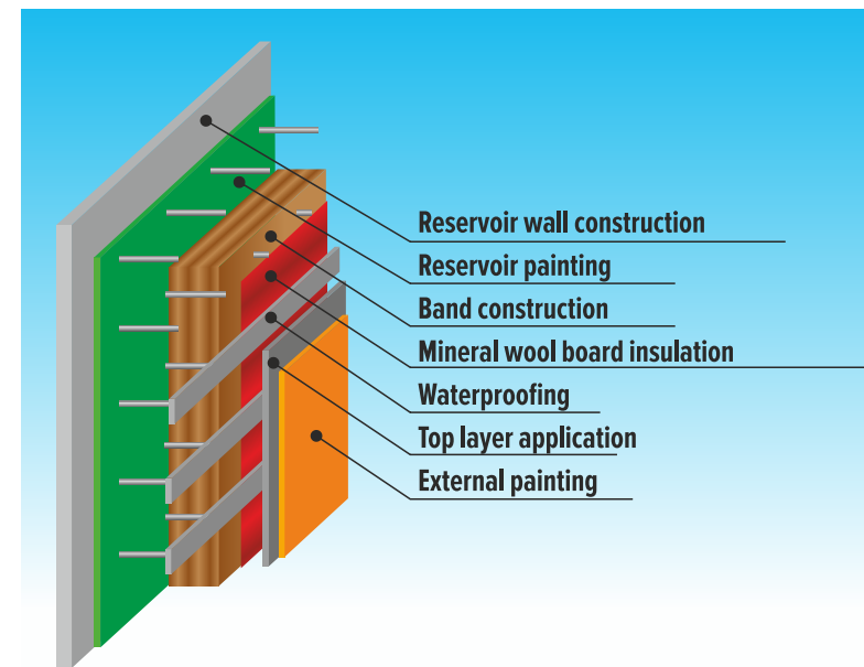
Standard technique of reservoir insulation
